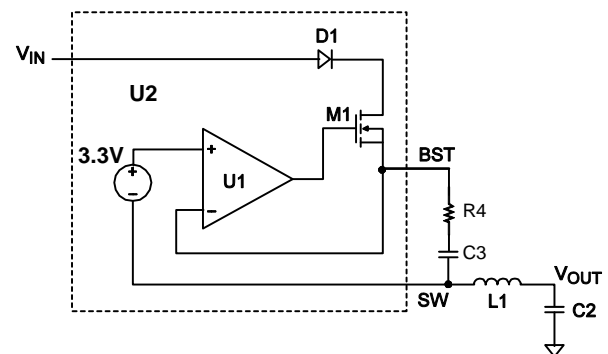
Figure 3: Internal Bootstrap Charger
